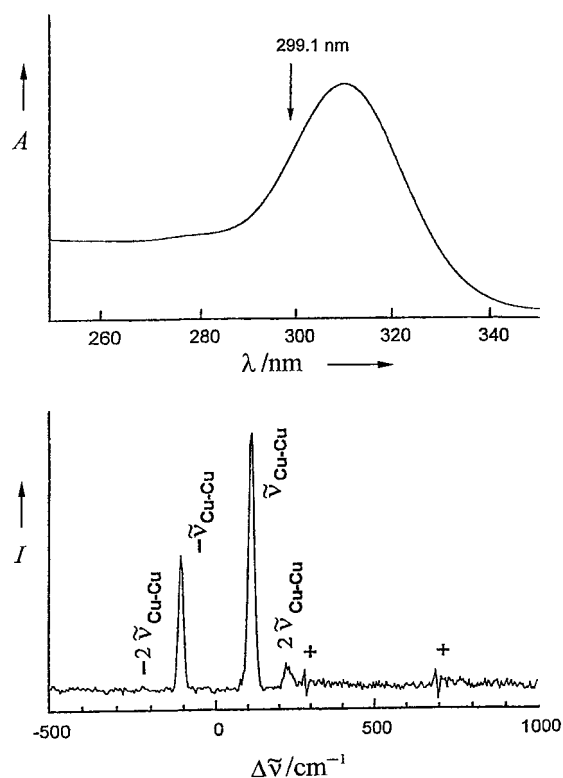
Figure 2. UV/Vis absorption spectrum of 1 (top) and resonance Raman spectrum (bottom) of 1 with excitation at 299.1 nm in dichloromethane (solvent subtraction artifacts marked by +).
